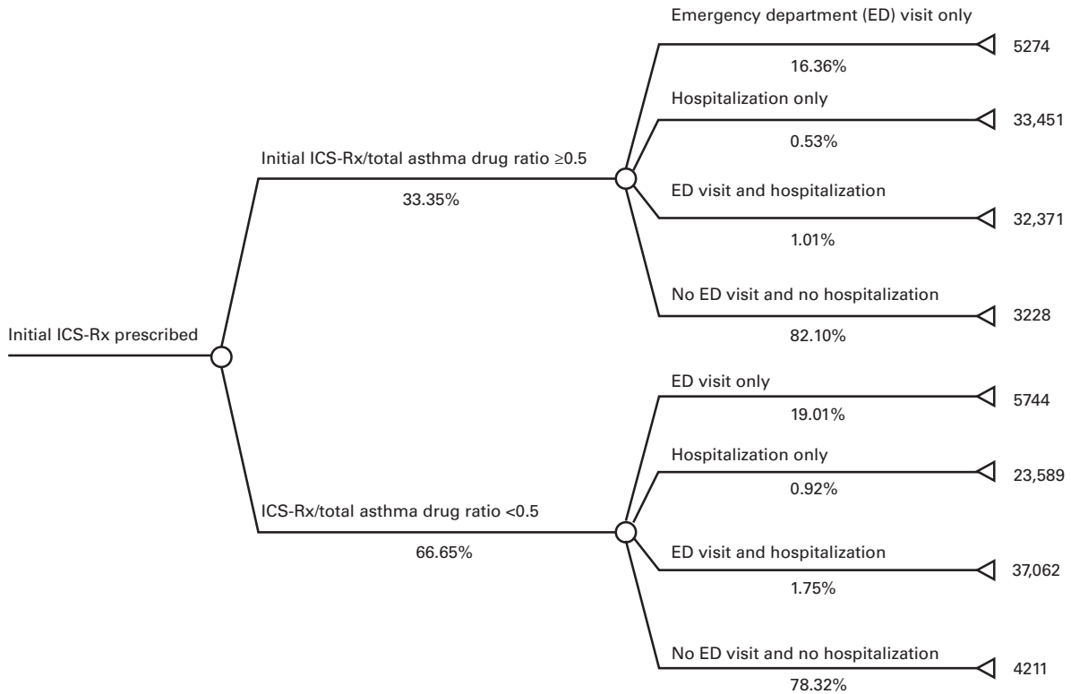
■ Figure. Model Structure of Decision Tree Analysis
