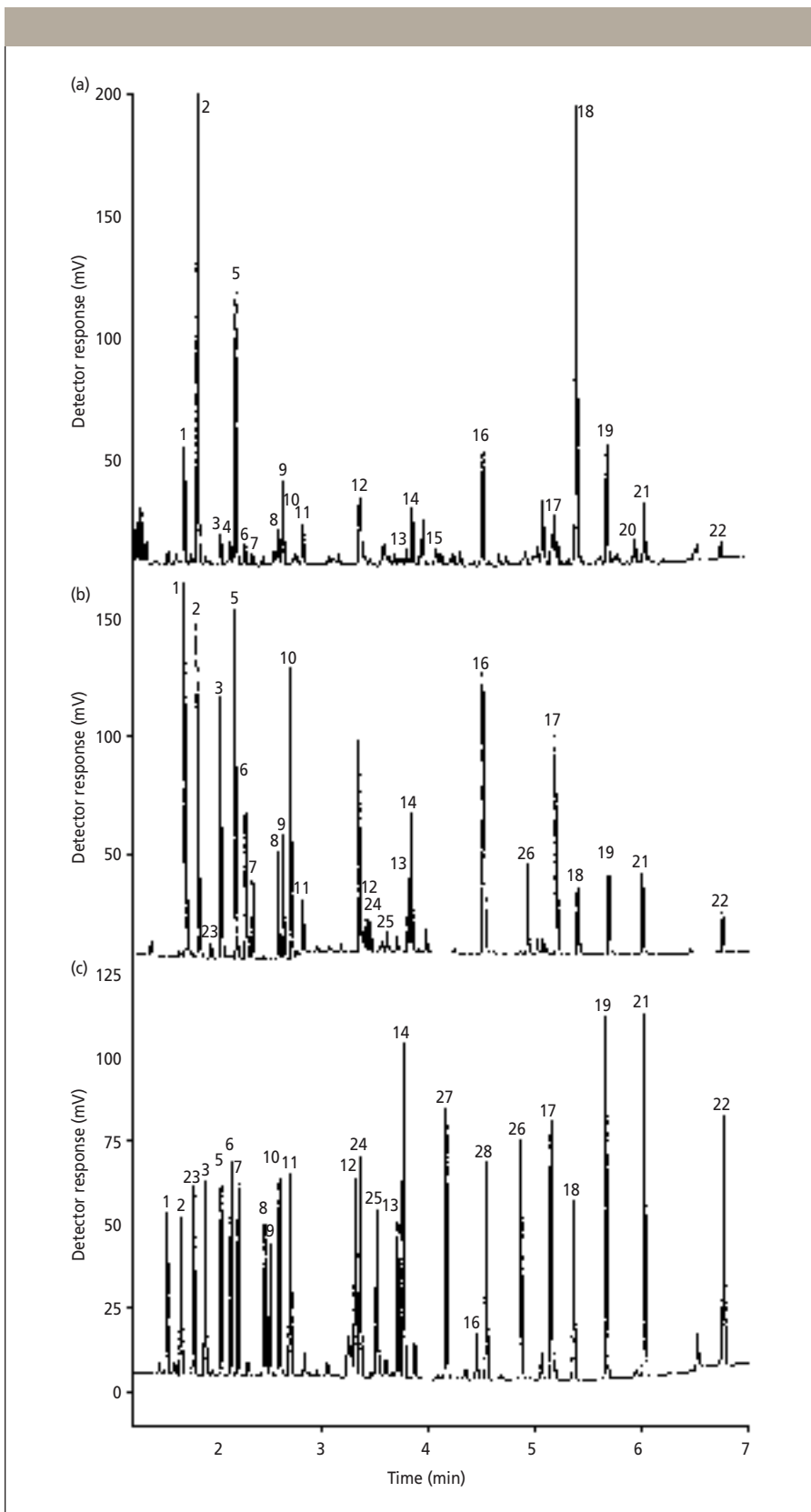
Figure 1: GC-flame ionization detection analysis of amino acids in 100 \mu L each of (a) urine and (b) serum and (c) amino acid standards (equimolar concentration). Column: Zebtron Amino Acid GC; oven temperature program: 110–320 ^{\circ} C at 30 ^{\circ} C/min. Peaks: 1 = alanine, 2 = glycine, 3 = valine, 4 = \beta -aminoisobutyric acid, 5 = norvaline (internal standard), 6 = leucine, 7 = isoleucine, 8 = threonine, 9 = serine, 10 = proline, 11 = asparagine, 12 = aspartic acid, 13 = glutamic acid, 14 = phenylalanine, 15 = \alpha -aminoadipic acid, 16 = glutamine, 17 = lysine, 18 = histidine, 19 = tyrosine, 20 = proline–hydroxyproline dipeptide, 21 = tryptophan, 22 = cystine, 23 = \alpha -aminobutyric acid, 24 = methionine, 25 = hydroxyproline, 26 = ornithine, 27 = cysteine, 28 = homocysteine.
