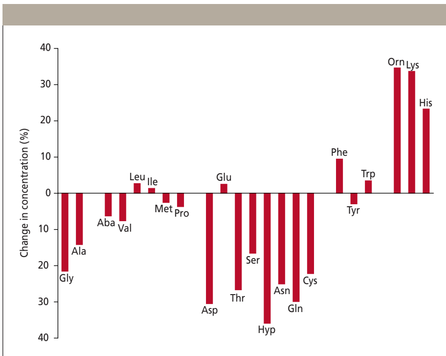
Figure 5: Changes in plasma amino acid yields after deproteinizing plasma with 10% and 3% ( y = 0 ) aqueous trichloroacetic acid. Values on the y axis represent altered yields found with the use of 10% trichloroacetic acid compared with 3% trichloroacetic acid.
