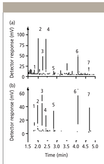
Figure 2: GC-flame ionization detection analysis of S-amino and aromatic acids (a) in human plasma and (b) corresponding standards. Column: Zebtron Amino Acid GC; oven temperature range: 140–300 ^{\circ} C. Peaks: 1 = methionine, 2 = ethionine (internal standard at 200 \mu mol/L), 3 = phenylalanine, 4 = cysteine, 5 = homocysteine, 6 = tyrosine, 7 = tryptophan.
