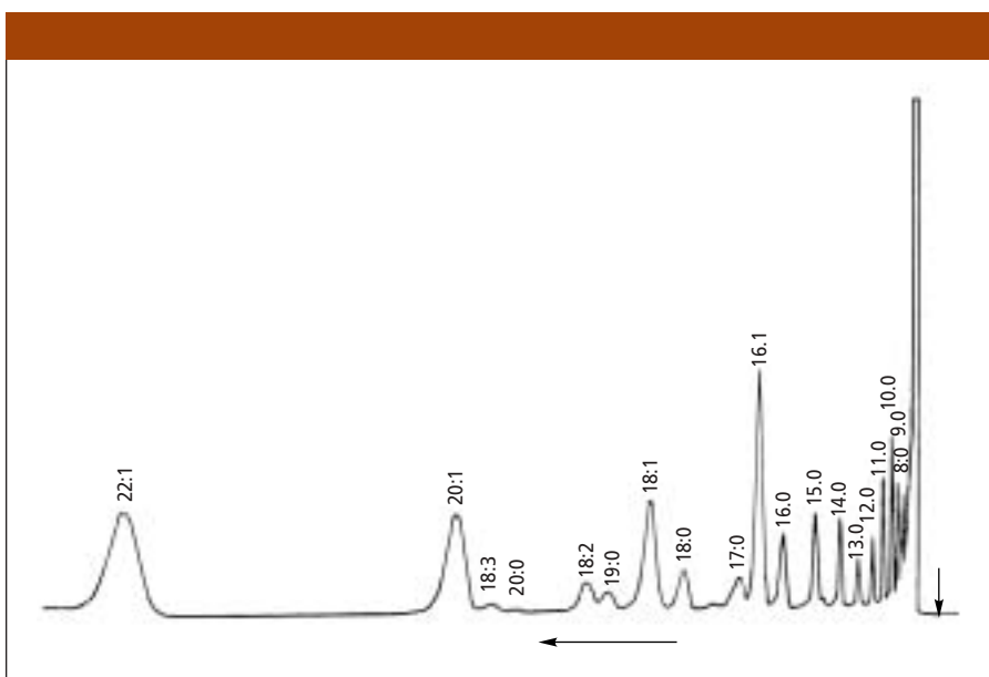
Figure 4: Chromatogram of fatty acid methyl esters, from 1964 (16). 10 ft \times \frac{1}{8} in. o.d. packed column containing 10% ethylene glycol cyanoethyl succinate on silanized support. Temperature: 194 °C; flame ionization detector.
