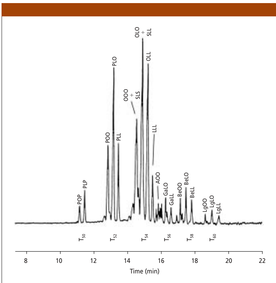
Figure 5: Chromatogram of the triglycerides of peanut oil from 1986 (20). 15 m × 0.25 mm fused-silica capillary column coated with bonded phenyl (65%) methyl silicone stationary phase ( d_f = 0.1\text{-}\mu\text{m} ). Column temperature programmed from 300 °C to 360 °C at 4 °C/min. Programmed-temperature vaporizer, heated from 50 °C to 400 °C. Sample: 0.5 \mu\text{L} of a 20- \mu\text{g}/\text{mL} solution in isooctane, split 1:50. Carrier gas: hydrogen. Flame ionization detector. The T numbers give the total carbon number of the three fatty acids in the triglyceride. The individual fatty acids are indicated by the following code: P = palmitic acid (16:0); S = stearic acid (18:0); O = oleic acid (18:1, cis ); L = linoleic acid (18:2, cis-cis ); A = arachidic acid (20:0); Ga = gadoleic acid (20:1, cis ); Be = behenic acid (22:0); Lg = lignoceric acid (24:0).
