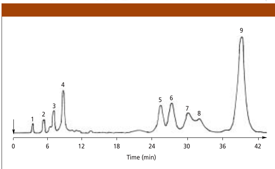
Figure 6: Packed column chromatogram of peppermint oil of Yakima Valley from 1958 (28). Isothermal conditions, thermal conductivity detector. Peaks: 1 = \alpha -pinene; 2 = \beta -pinene; 3 = limonene; 4 = eucalyptol; 5 = menthone; 6 = menthofuran, 7 = menthyl acetate; 8 = unknown, 9 = menthol.
