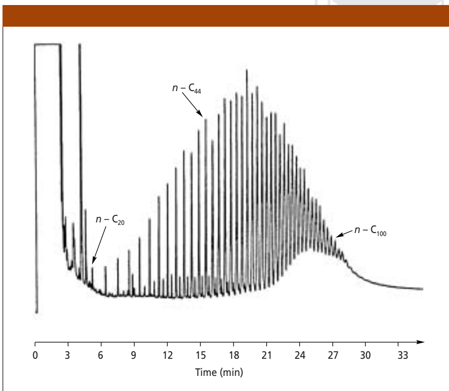
Figure 3: Chromatogram of a Polywax 1000 sample containing hydrocarbons with carbon numbers as large as C_{100+} , from 1987 (9). 8 m \times 0.25 mm aluminum-clad fused-silica capillary column coated with bonded methylsilicone stationary phase ( d_f = 0.1\text{-}\mu\text{m} ). Column temperature programmed from 50 °C to 430 °C at 15 °C/min. Programmed-temperature vaporizer, heated from 50 °C to 440 °C. Sample: 0.5 \mu\text{L} of a 1-mg/mL solution in 1:1 \text{CS}_2 – n -decane, split 1:20. Carrier gas: hydrogen. Flame ionization detector.
