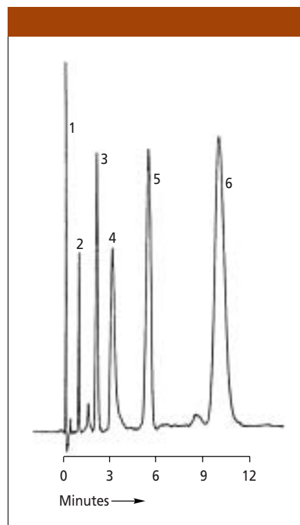
Figure 9: Chromatogram of a pesticide mixture from a 1963 advertisement of a gas chromatograph with an electron-capture detector (37). 2 ft × 3 mm glass packed column containing 2.5% SF 96 methylsilicone on silanized support. Column temperature: 180 °C. Sample volume: 0.5 μL (liquid). Peaks: 1 = solvent ( n -heptane); 2 = lindane; 3 = parathion; 4 = sulphenone; 5 = ethion; 6 = EPN. Sample concentration was in the nanogram-per-microliter (ppm) range.
