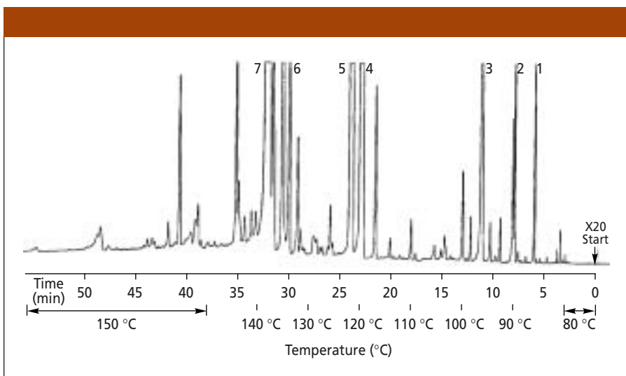
Figure 7: Capillary chromatogram of peppermint oil of Yakima Valley from 1962 (29). 150 ft \times 0.25 mm stainless steel capillary column coated with Ucon Oil 50-HP-2000 poly(propylene glycol). Sample volume: 1 \mu L (liquid), split. Flame ionization detector. Major peaks: 1 = \alpha -pinene; 2 = \beta -pinene; 3 = eucalyptol; 4 = menthone; 5 = menthofuran; 6 = menthyl acetate; 7 = menthol.
