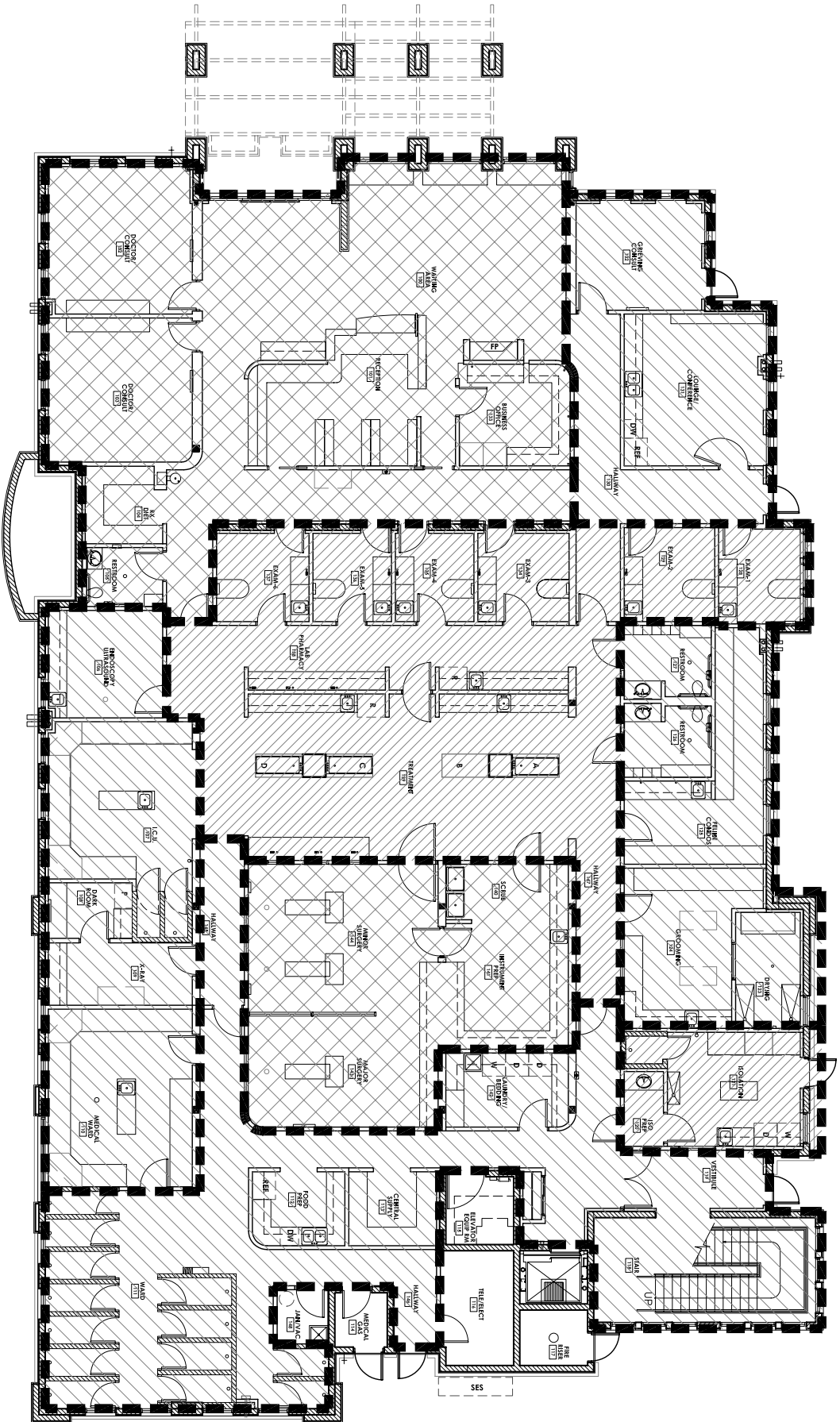
FIRST FLOOR HVAC ZONES EXHIBIT
