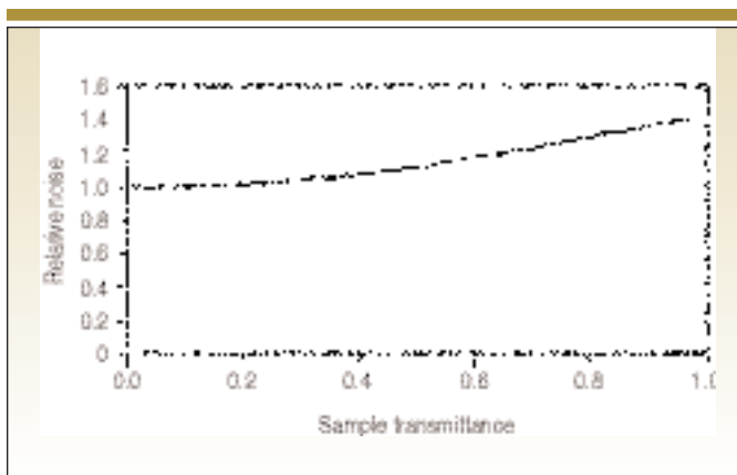
Figure 1. Noise level of a transmittance spectrum as a function of the sample transmittance.
