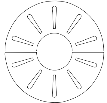
ALCORQUE Tree Pit | Cuvette d'arbre BALI PLUS+ BLUE Ø100 cm Ø39.3" COD. P183
