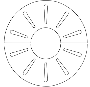
ALCORQUE Tree Pit | Cuvette d'arbre BALI PLUS+ SAND Ø100 cm Ø39.3" COD. P183
