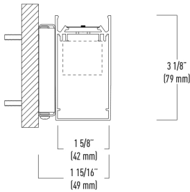
RW13-V / Frosted Flush Lens
