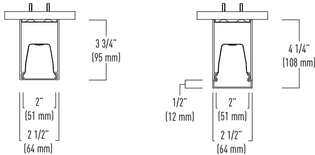
RR24-D / Frosted Flush Lens
