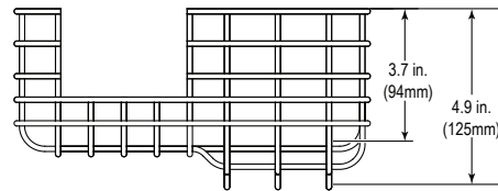
STI-9720 TOP VIEW
