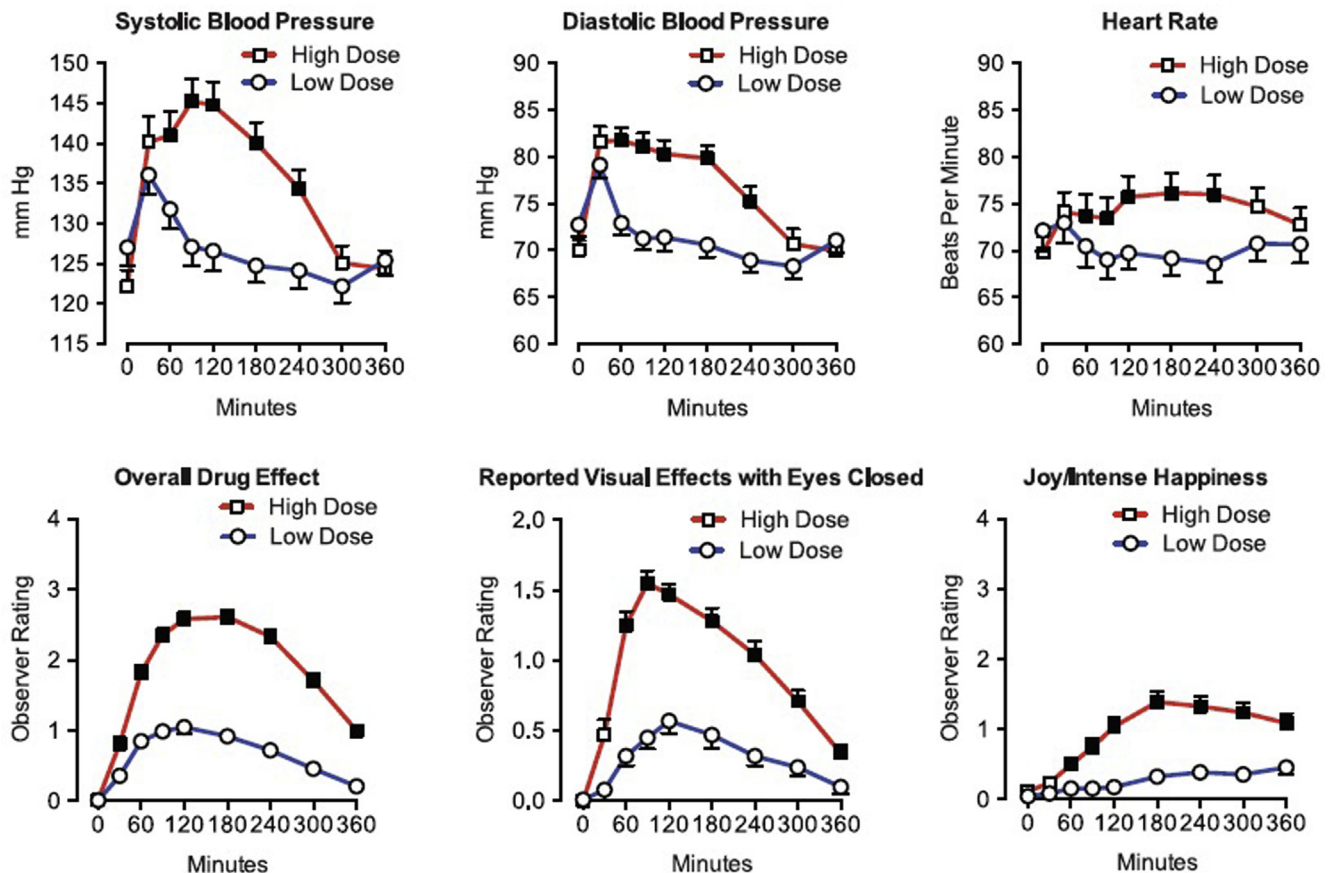
Fig. 2. Cardiovascular and observer-rated effects of oral psilocybin in cancer patients ( n = 50 ). Each panel shows the mean ( \pm SEM) within-subject time-course effect of a moderately-high ( \sim 0.314 or \sim 0.429 mg/kg) versus low, placebo-like ( \sim 0.014 or \sim 0.043 mg/kg) dose of psilocybin. For observer ratings, the Y-axis spans the range of possible scores. Filled squares indicate that planned comparisons showed the high dose condition significantly differed from the low dose condition at that time-point ( p < 0.05 ). Figure from Griffiths et al. (2016), Fig. 2).
