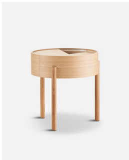
110497 Arc side table White pigmented lacquered oak Diameter 420 mm / 16.5 " Height 450 mm / 17.7 "
