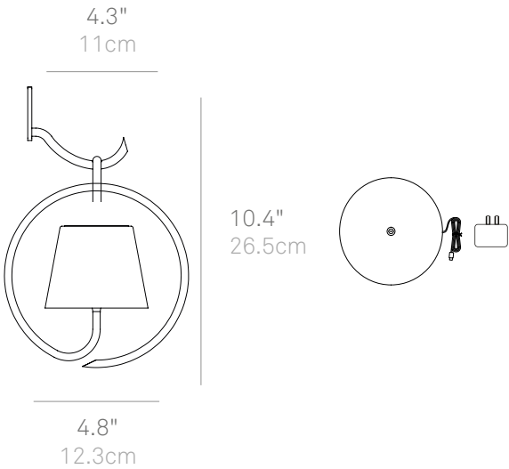
LD0689 Wall sconce with mounting hook and ring
