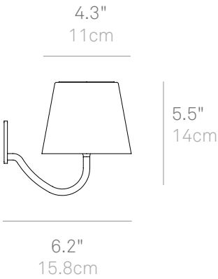
LD0688 Wall sconce with mounting bracket
