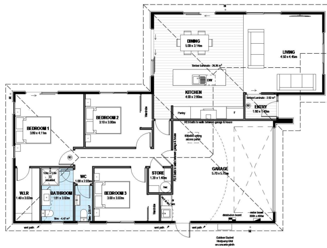
1 FLOOR PLAN 1:120
