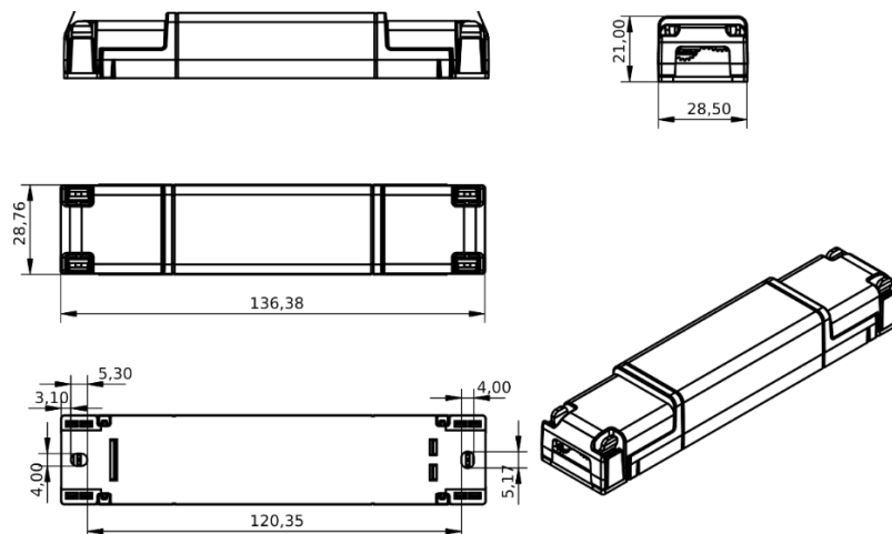
Figure 5: Mechanical Dimensions
