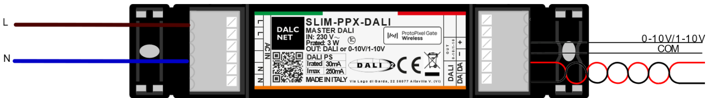
Figure 2: Wiring diagram
