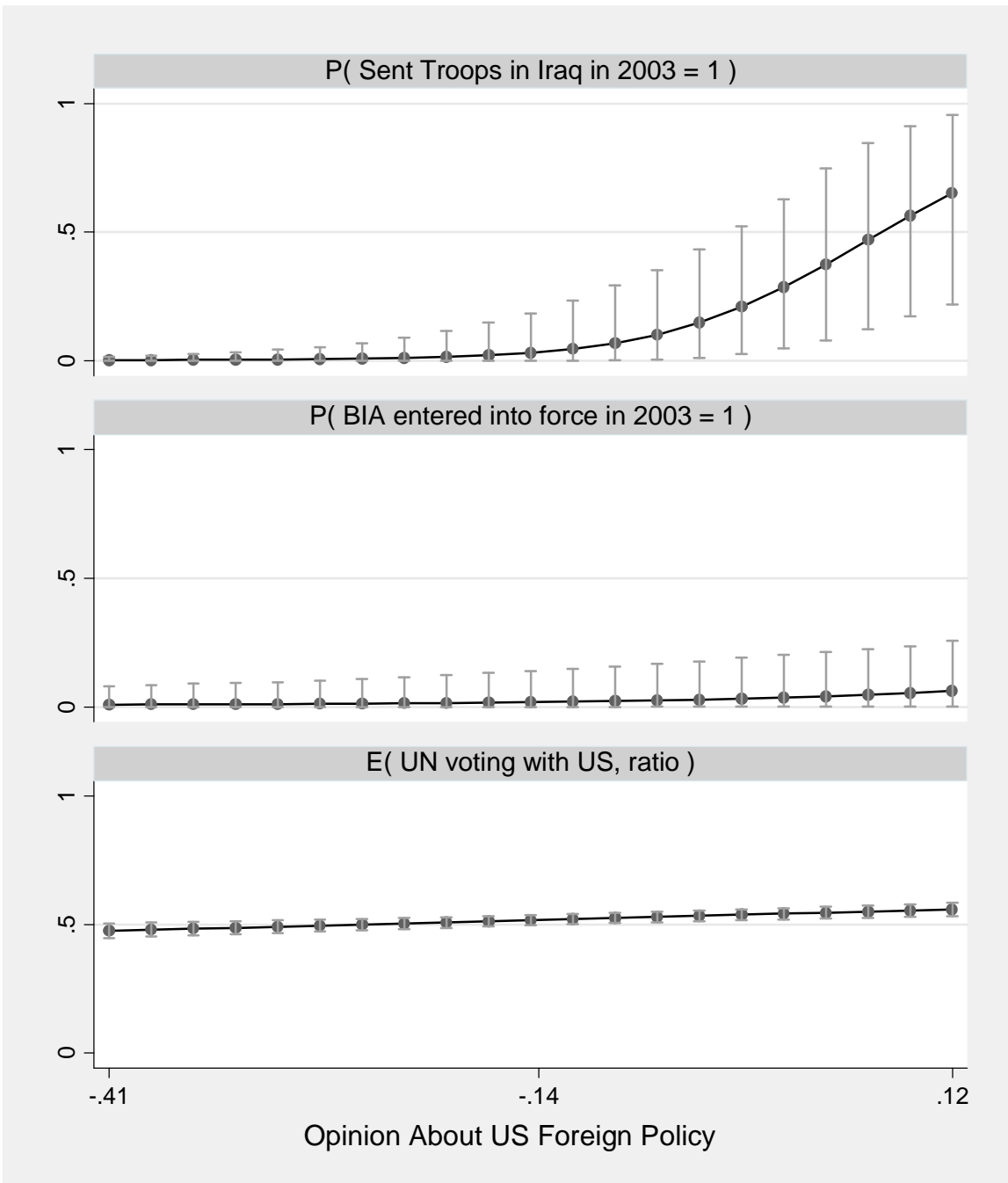
Figure 2: Marginal Effects
