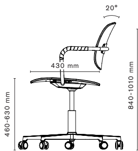
5-Star Swivel Base
