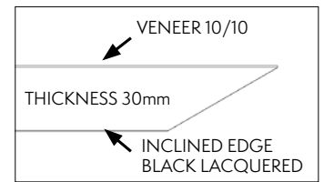
TOP SECTION
