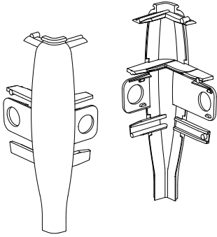
Vertiglide™ Valance Corner End Cap (Aluminum Valance only) See Sydney Corner Kits .
